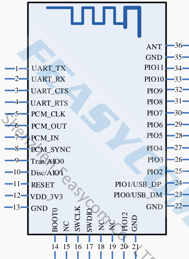
Figure 4: PIN description
