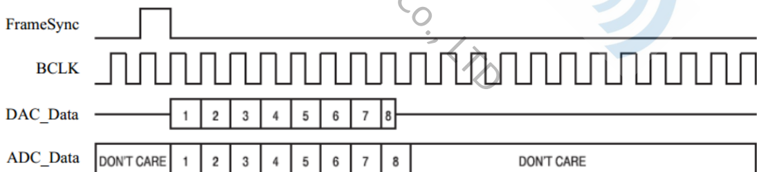
Figure 6: Short FrameSync
