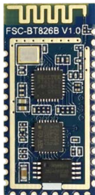
Figure 2: Module picture
