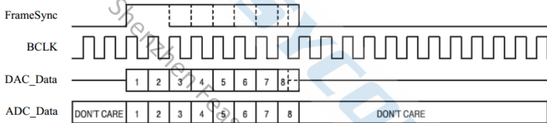
Figure 5: Long FrameSync
