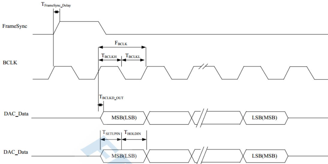
Figure 12: PCM Interface (Short FrameSync)
