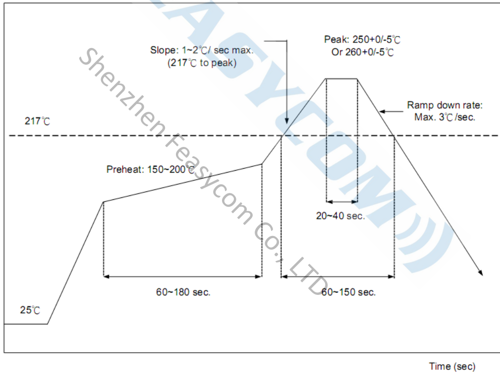
Figure 13: Typical Lead-free Re-flow Solder Profile
