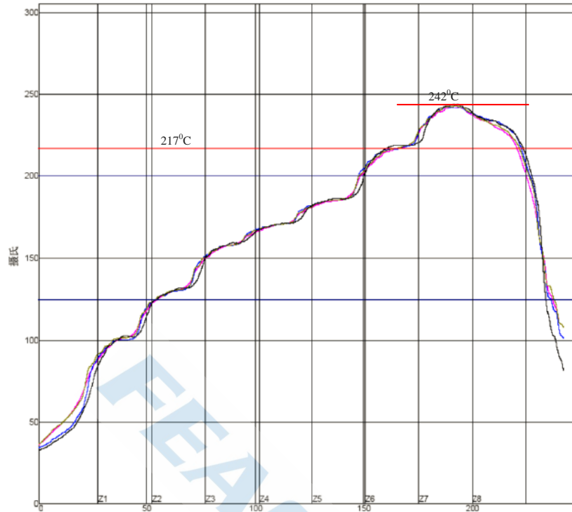
Figure 14 : Typical Lead-free Re-flow
