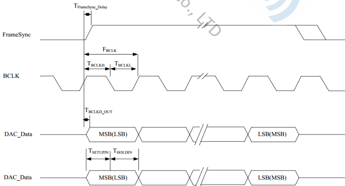
Figure 11: PCM Interface (Long FrameSync)
